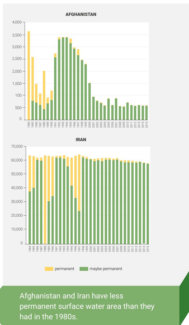
Figure 6: Annual changes in the spatial extent of open water bodies in Afghanistan and Iran
