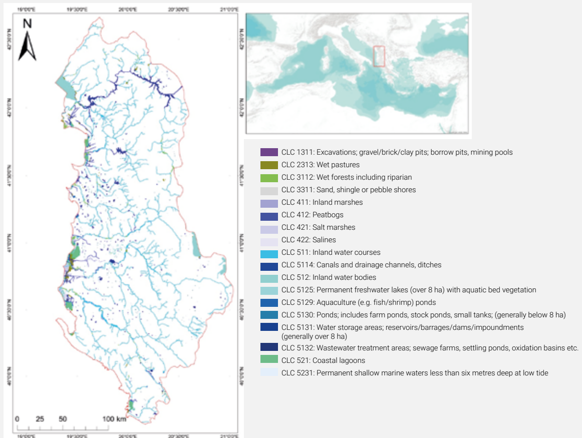
Figure 13: Identification of “effective” wetlands within the potential wetlands layer, using a LULC classification based on the CLC-Ramsar definitions
